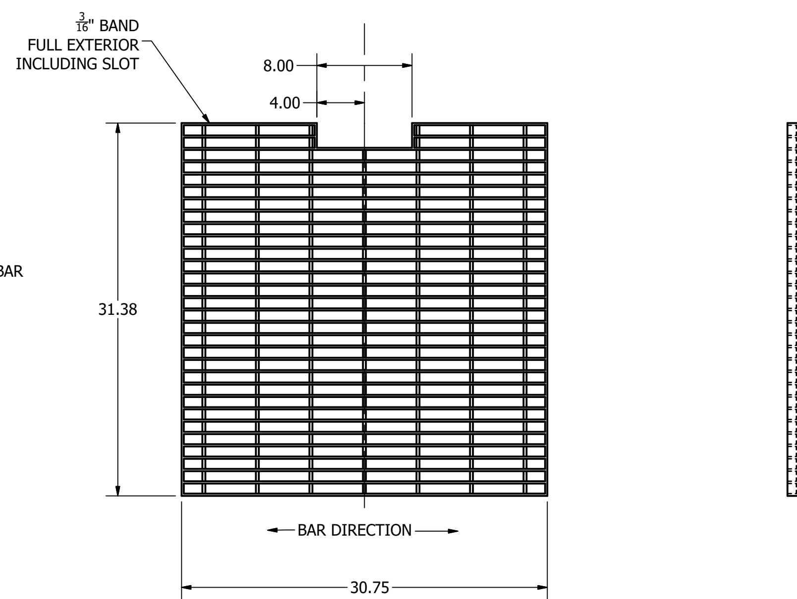
GRATING SCALE 1" = 0'-8"
