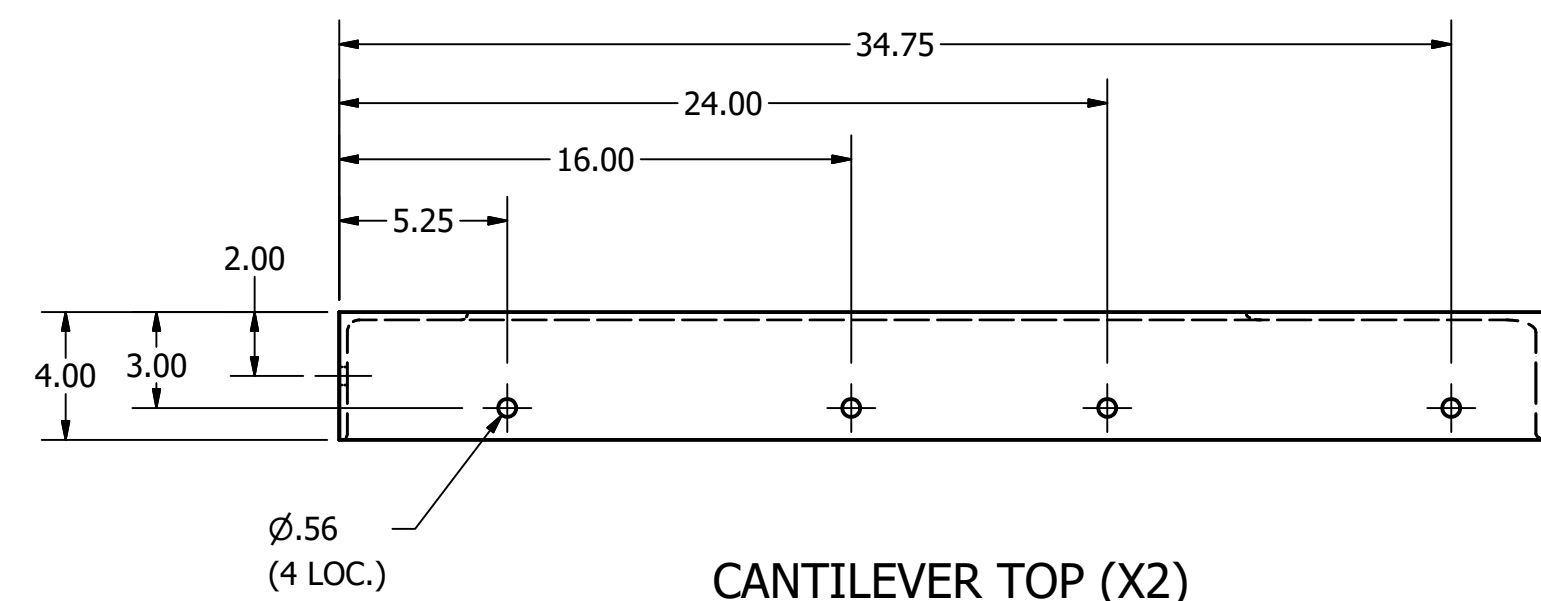
CANTILEVER TOP (X2) SCALE 1"=0'-6"
