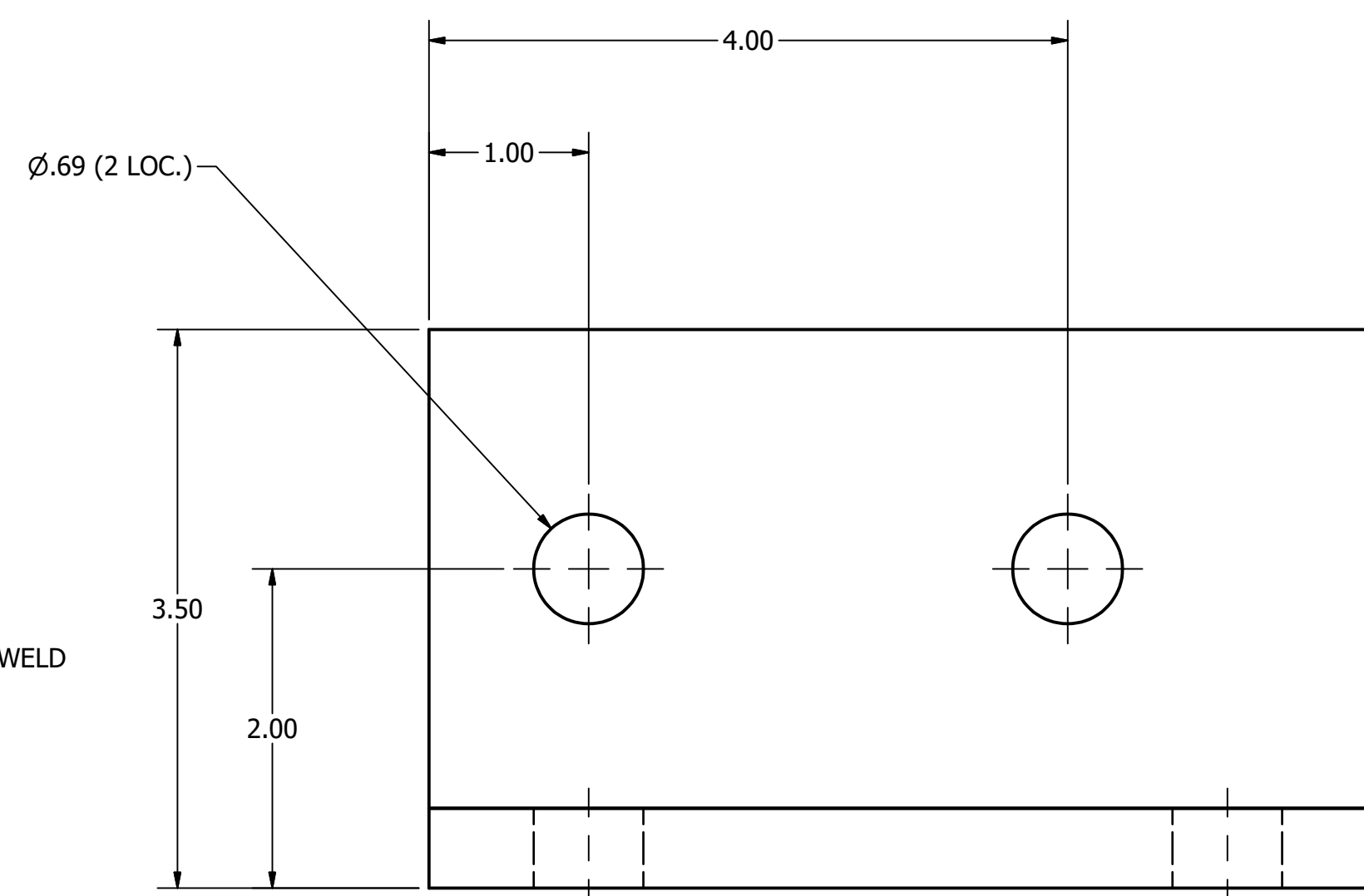
FRONT BOTTOM BRACKET SCALE 1"=0'-1"
