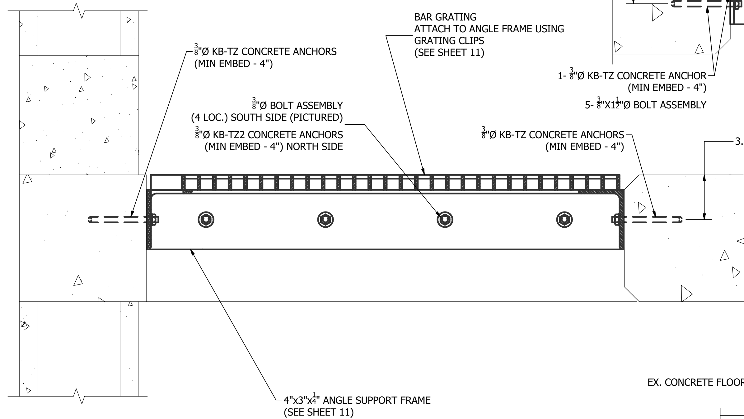
SECTION C-C
