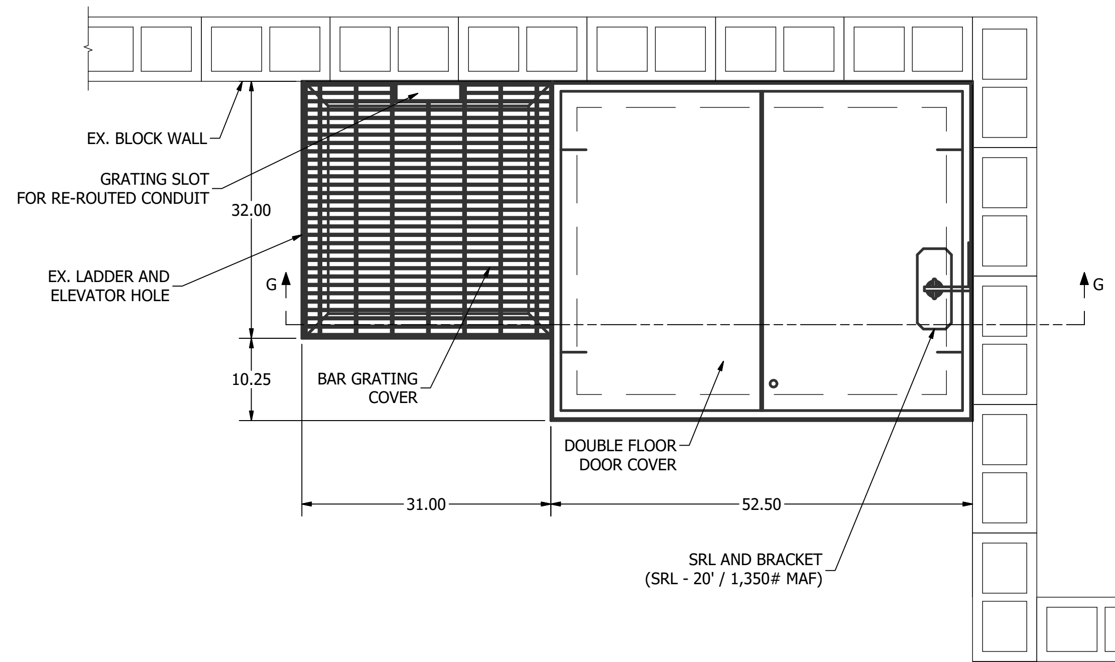
PLAN - TOP HATCH SCALE 1"=1'-0"
