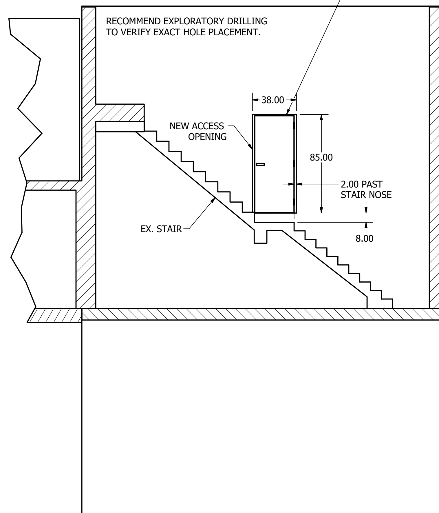
SECTION B-B SCALE 1"=4'-0"
