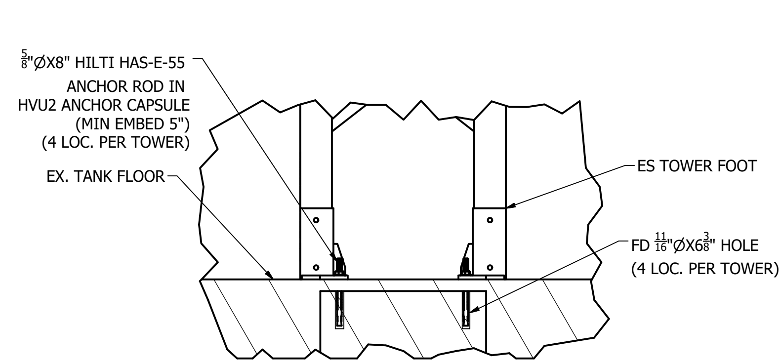
DETAIL P SCALE 1"=1'-0"
