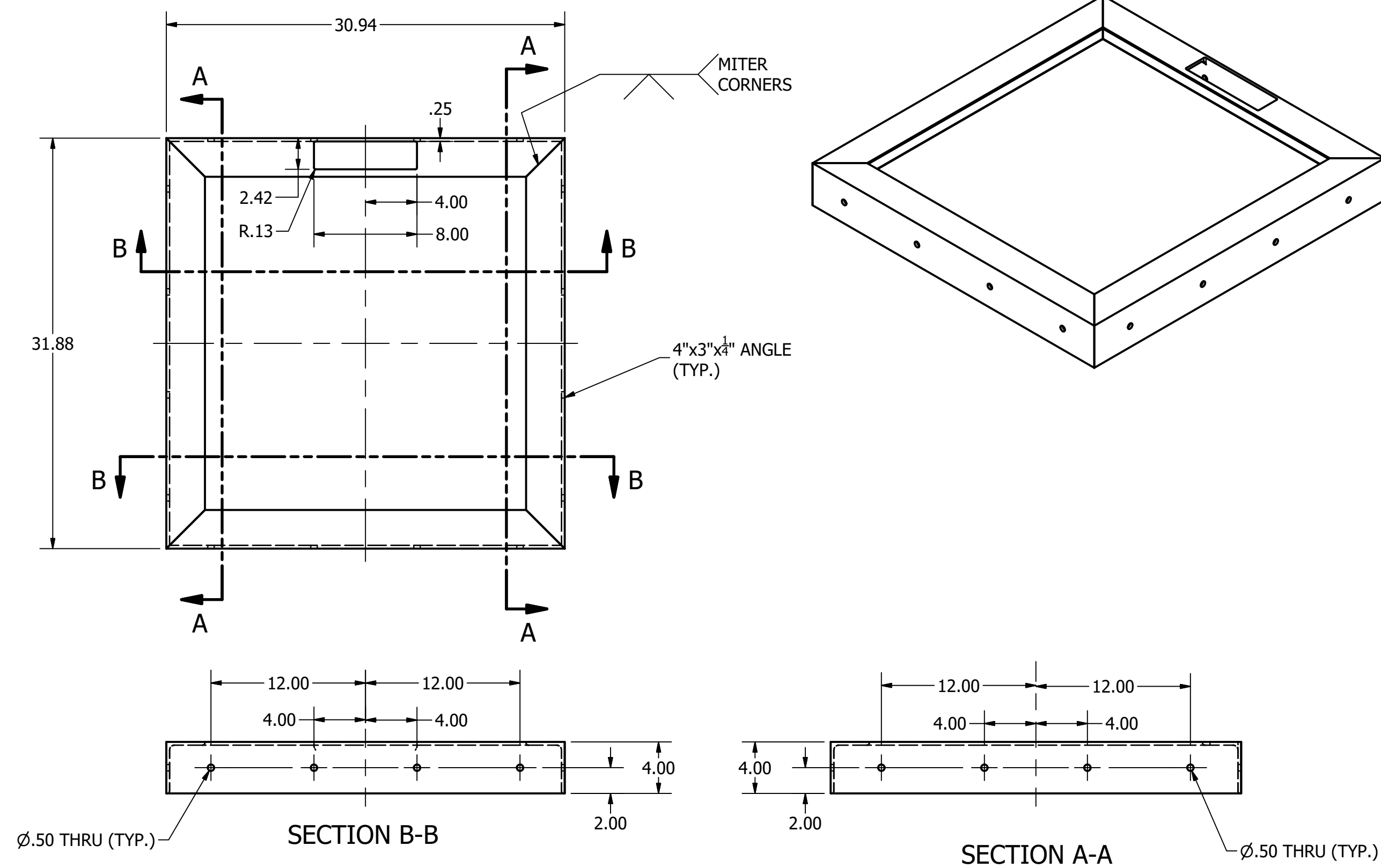
ANGLE SUPPORT FRAME SCALE 1"=0'-8"
