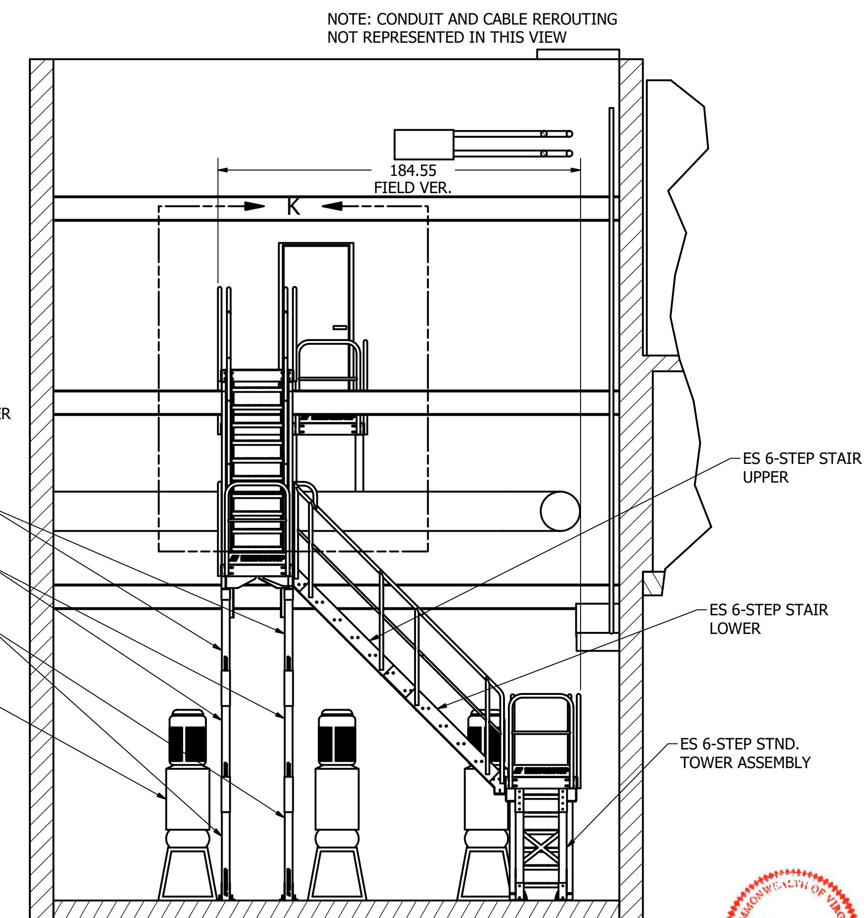
SECTION F-F SCALE 1"=4'-0"
