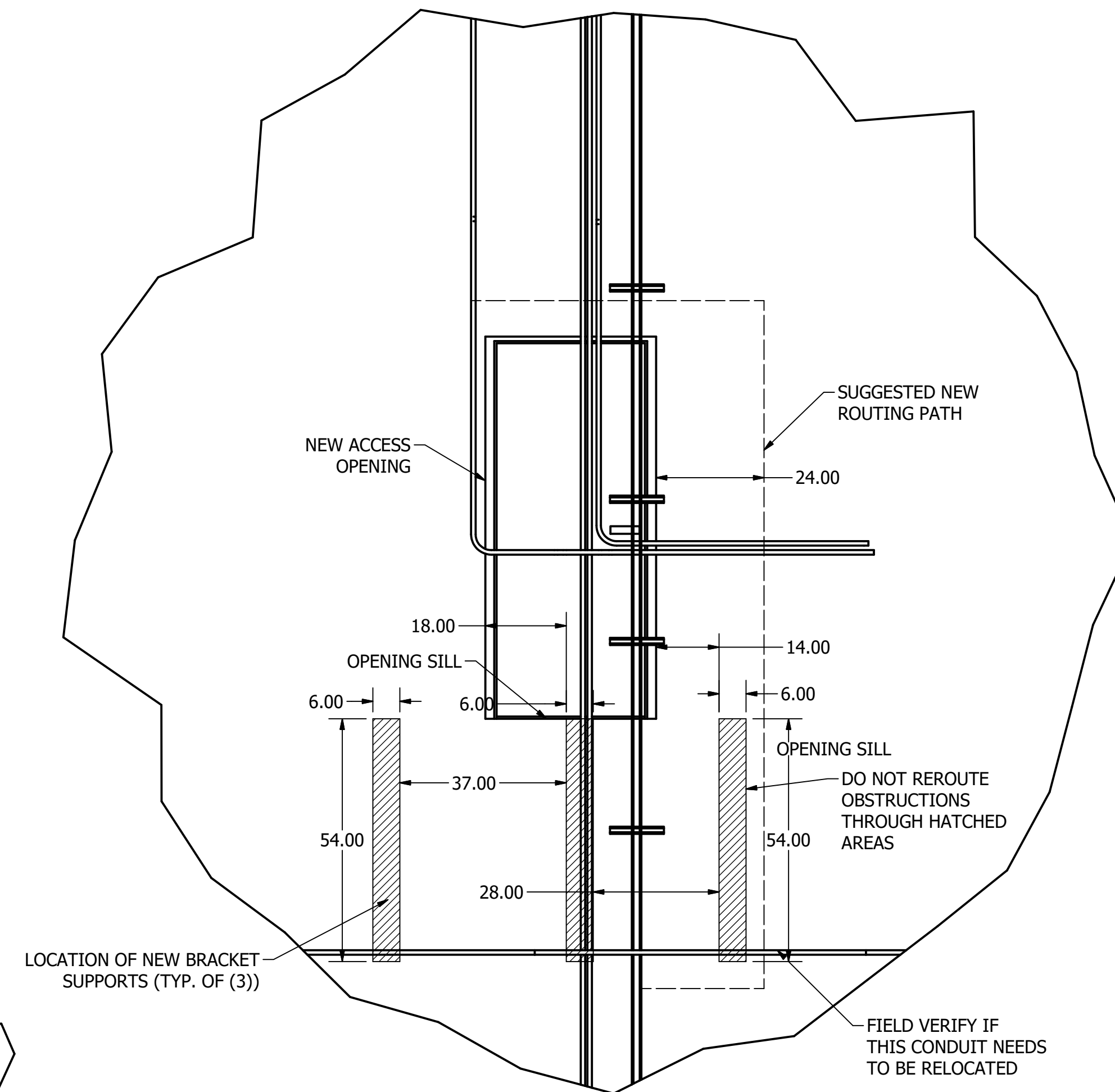
DETAIL D SCALE 1"=2'-0"
