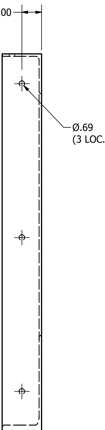
CANTILEVER FRONT (X2) SCALE 1"=0'-6"
