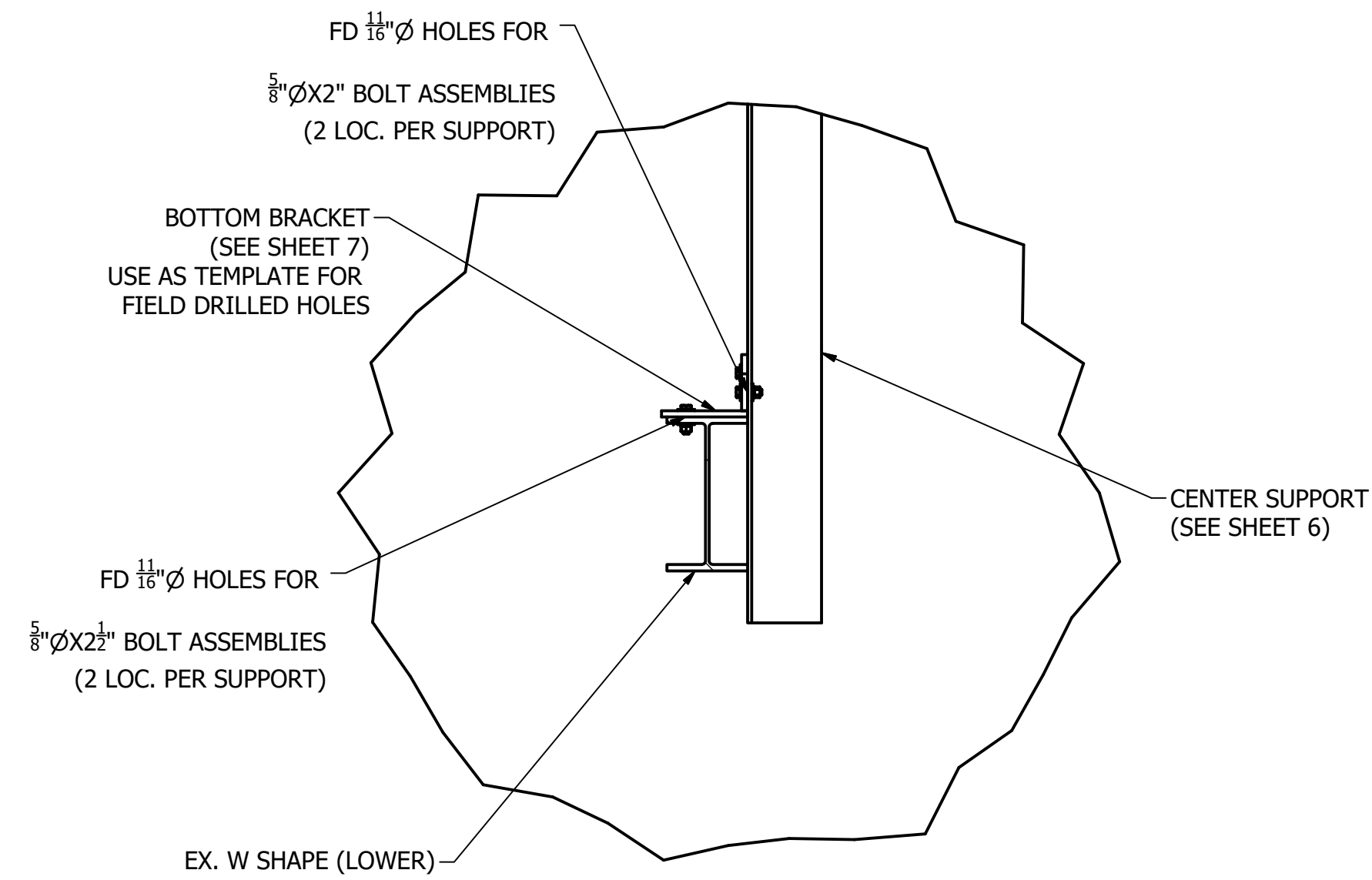
DETAIL R SCALE 1"=1'-0"
