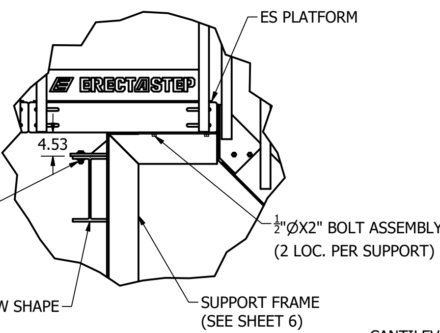
DETAIL M SCALE 1"=1'-6"
