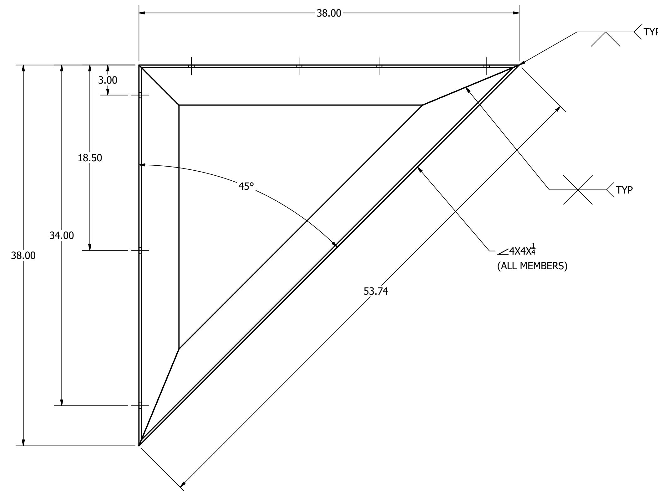
CANTILEVER SIDE (X2) SCALE 1"=0'-6"
