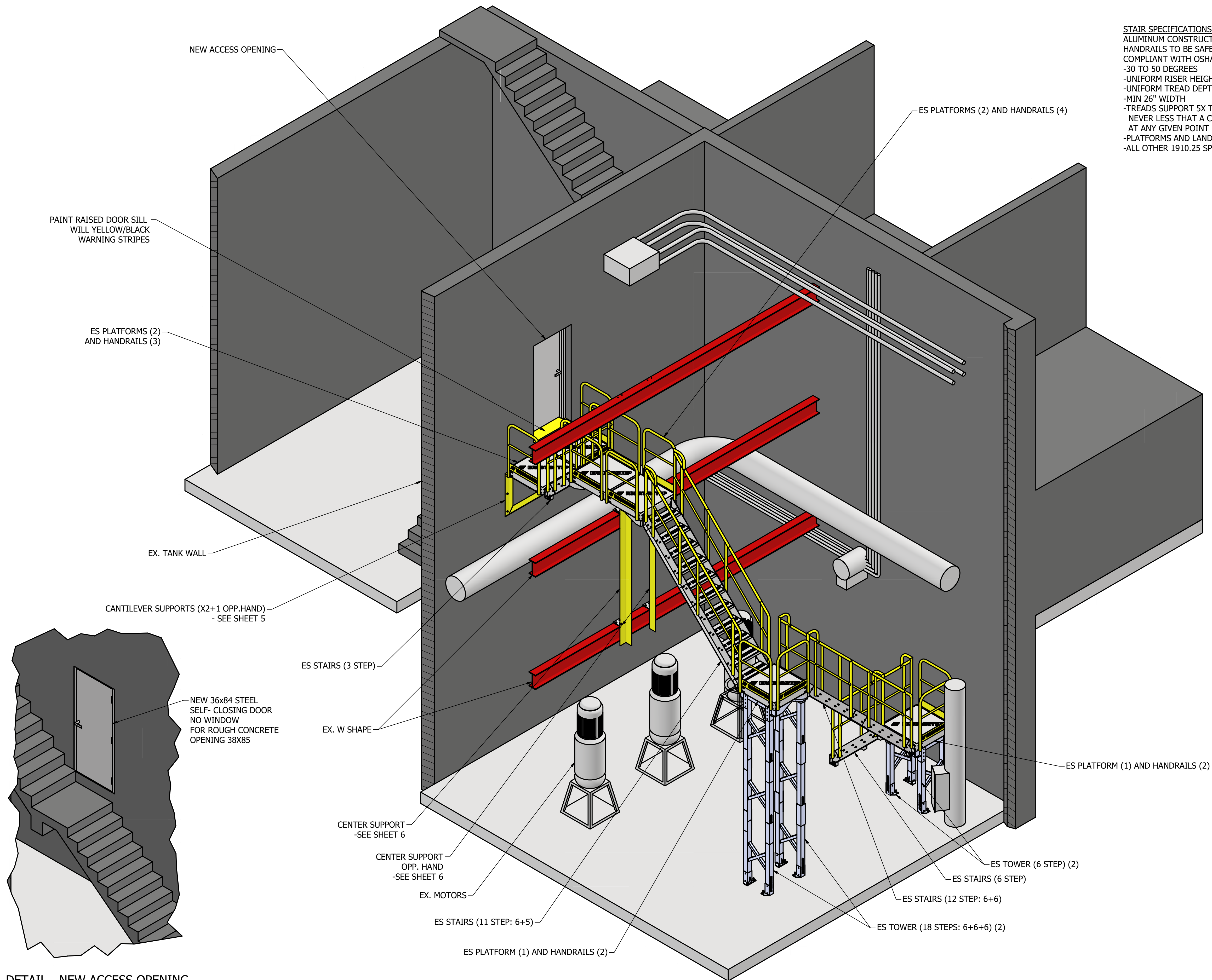
DETAIL - NEW ACCESS OPENING
