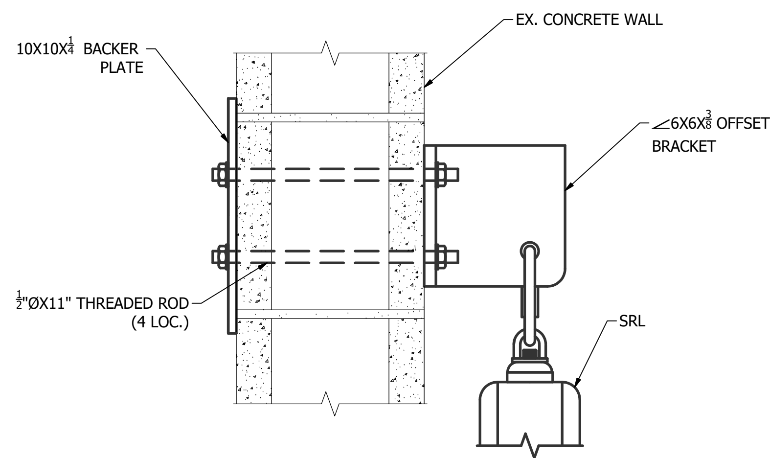
DETAIL - H-H SRL ATTACHMENT SCALE 1"=0'-4"
