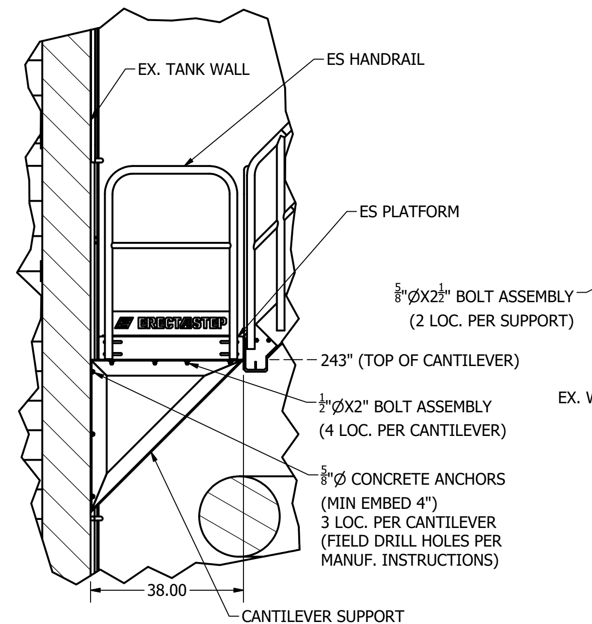
DETAIL L SCALE 1"=2'-0"
