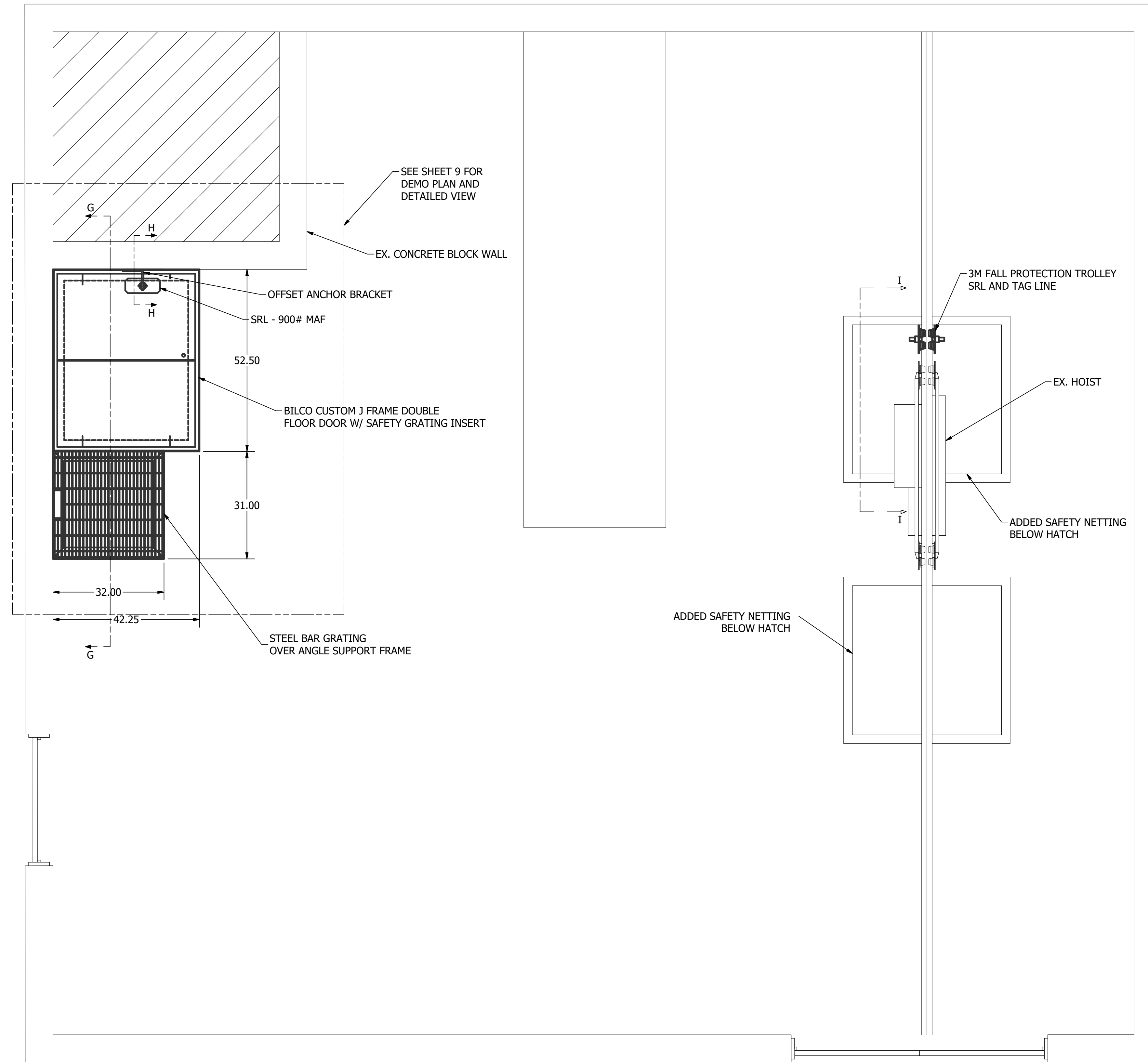
PLAN - TOP HATCHES SCALE 1"=1'-6"
