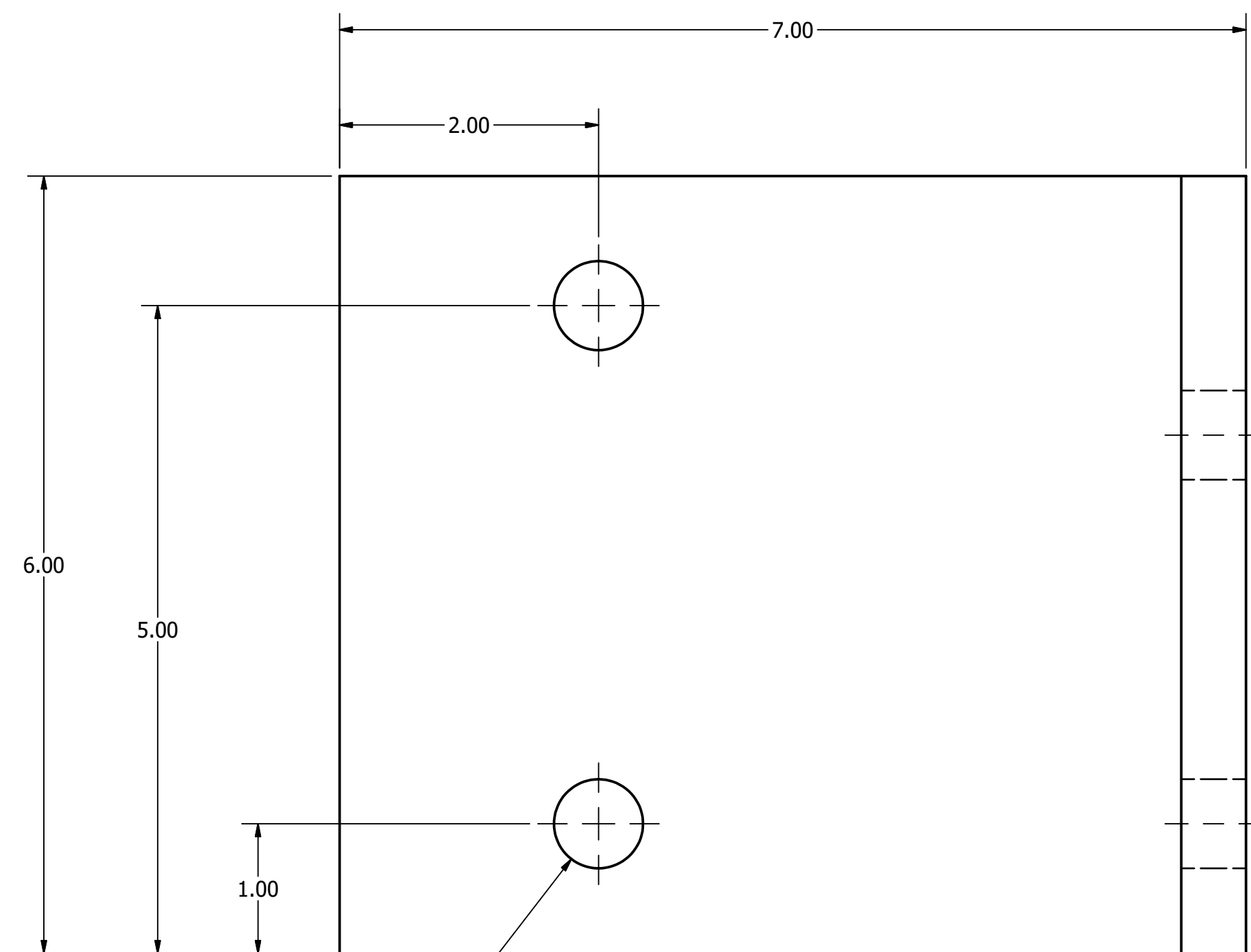
TOP BOTTOM BRACKET SCALE 1"=0'-1"
