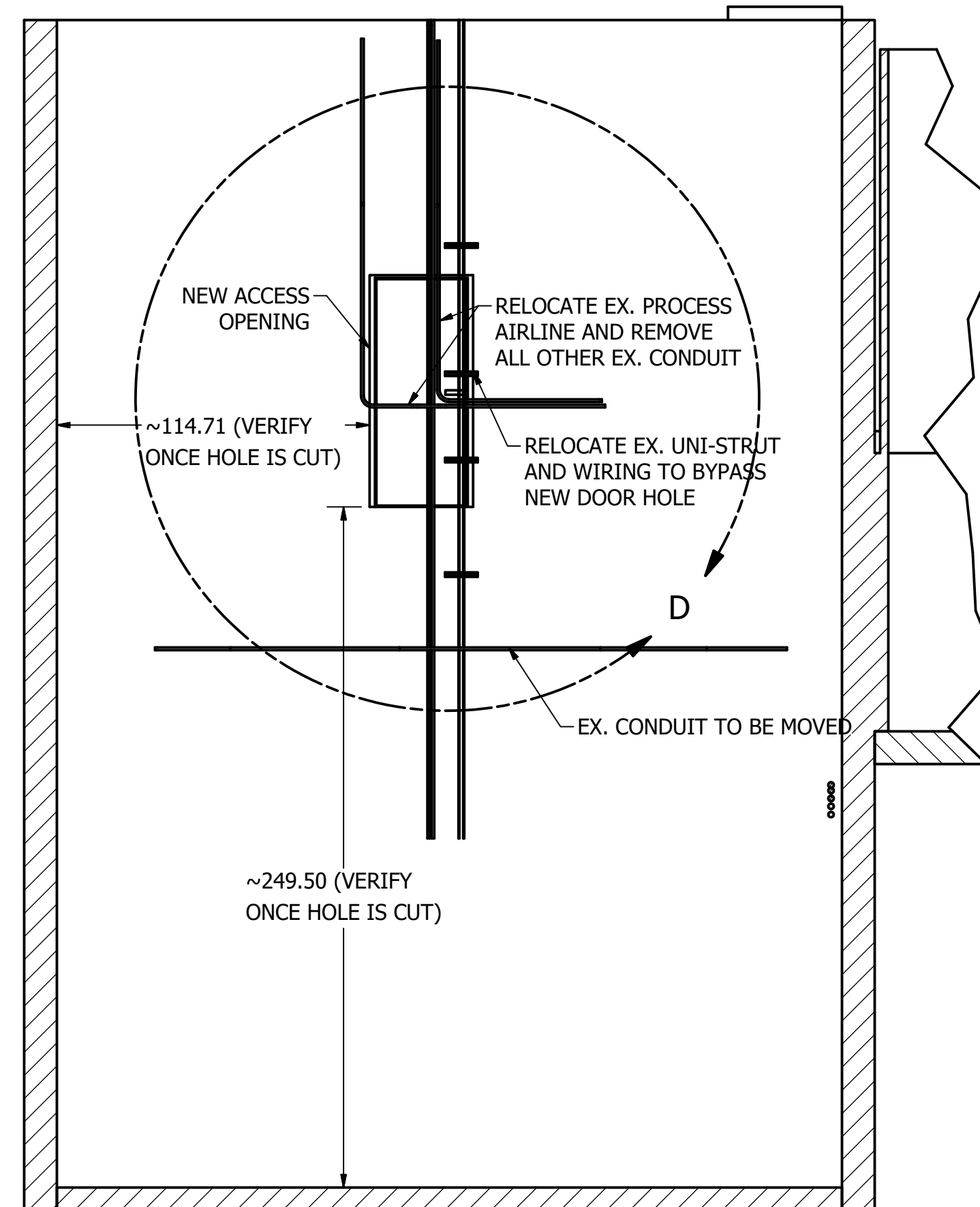
SECTION C-C SCALE 1"=4'-0"
