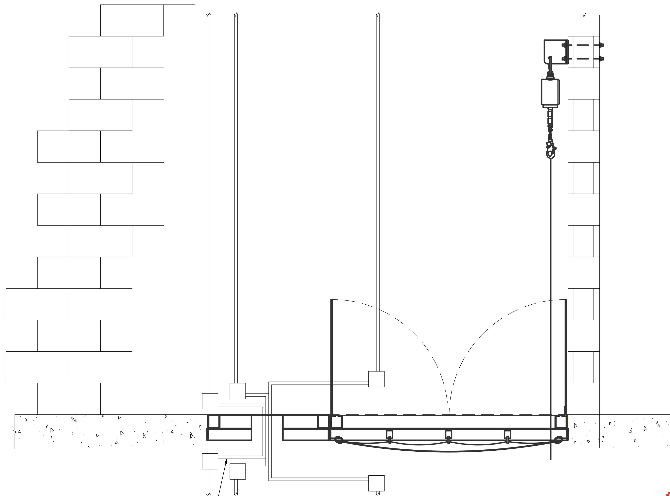
SECTION G-G - TOP HATCH SCALE 1"=1'-0"
