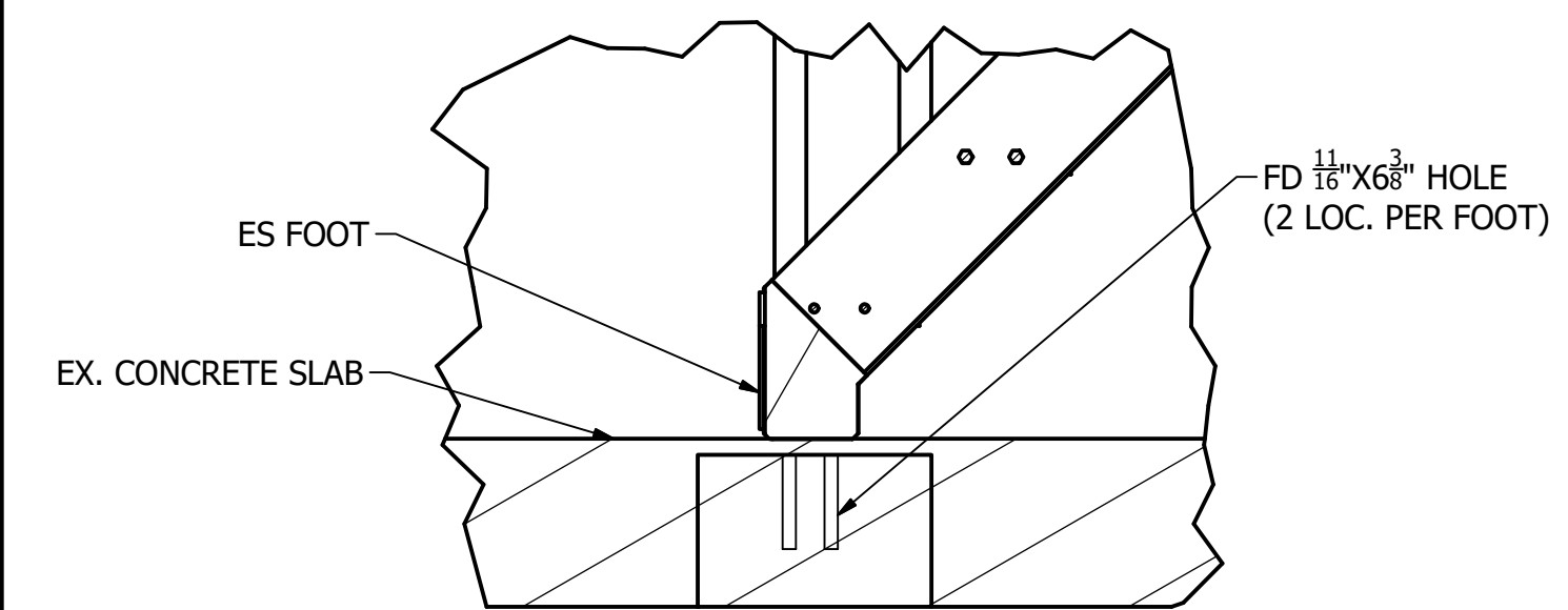
DETAIL J SCALE 1 / 12
