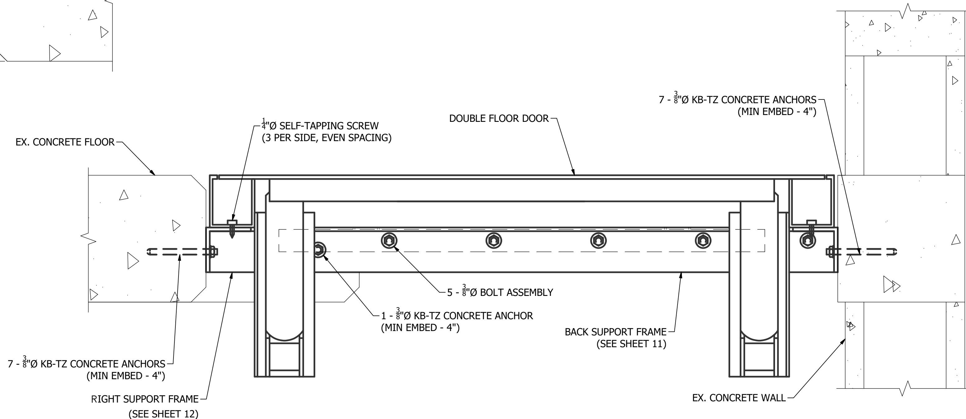
SECTION B-B
