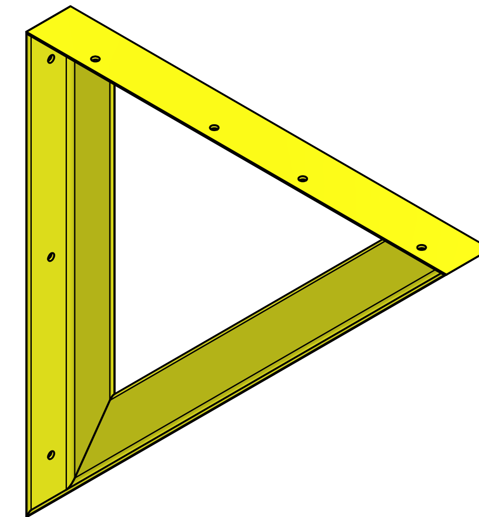
CANTILEVER ISO (X2) SCALE 1 / 6
