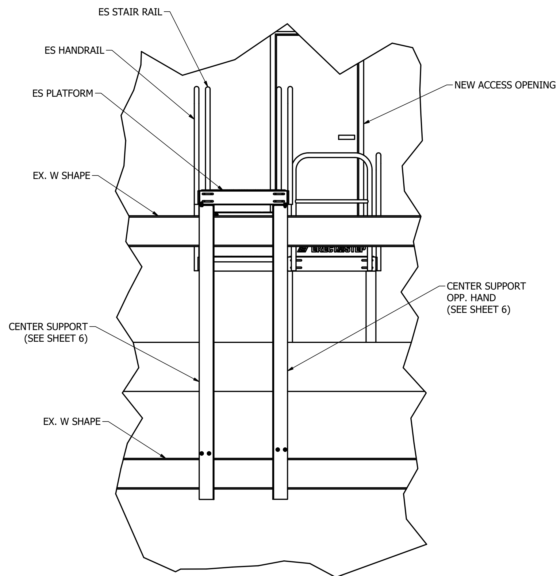
DETAIL Y-Y SCALE 1"=2'-0"
