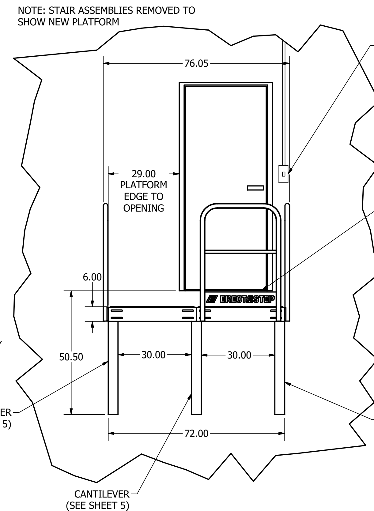
DETAIL K SCALE 1"=2'-0"
