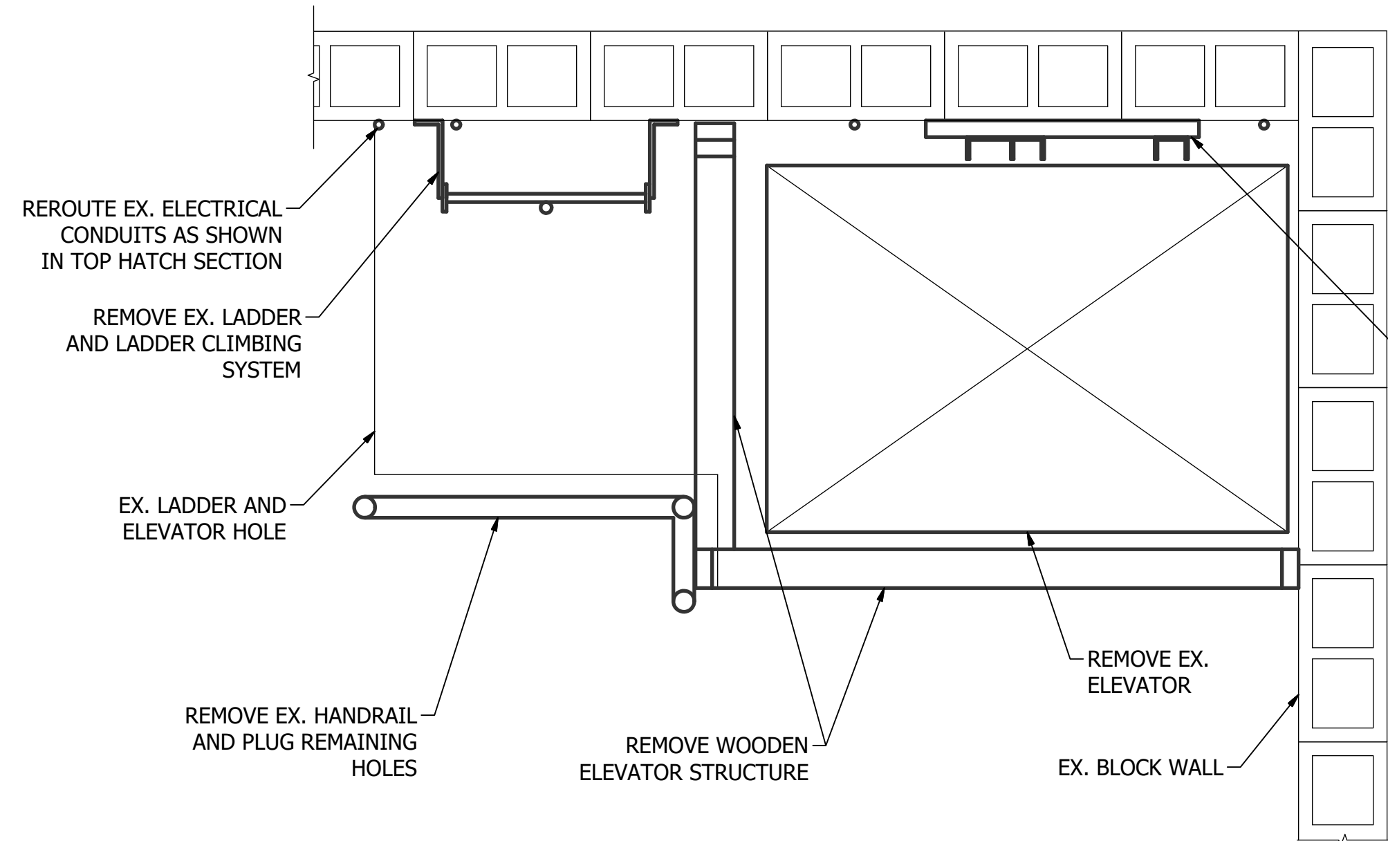
DEMO PLAN SCALE 1"=1'-0"
