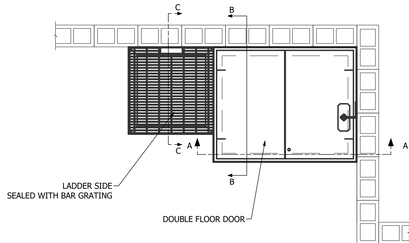
PLAN - NEW HATCH
