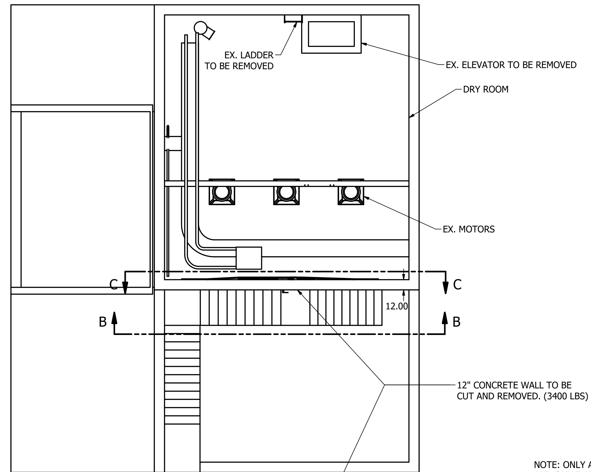
EX. TANK PLAN
