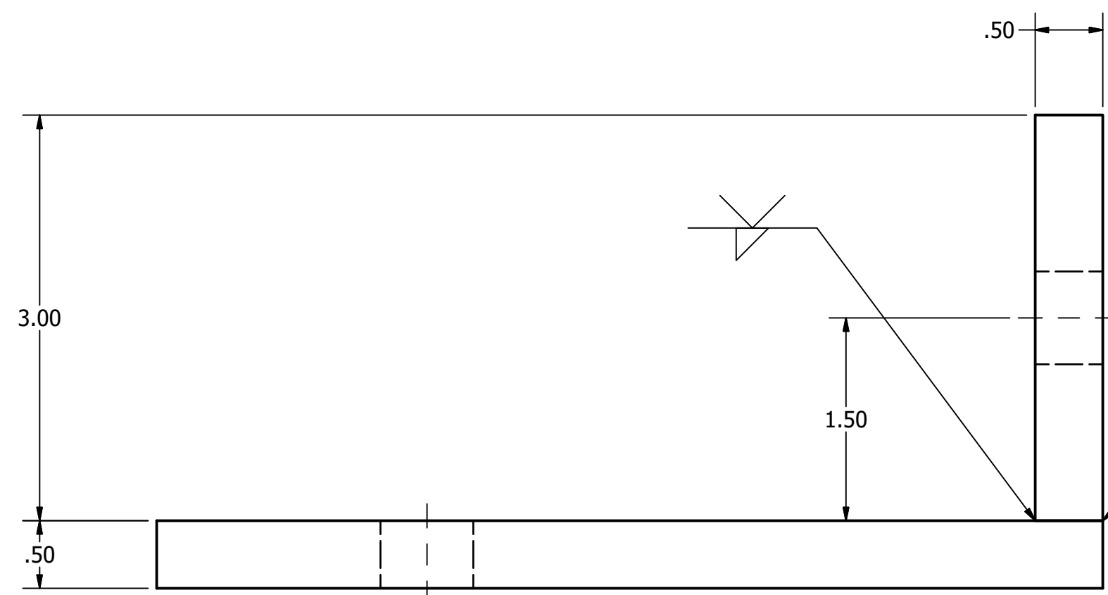
SIDE BOTTOM BRACKET SCALE 1"=0'-1"
