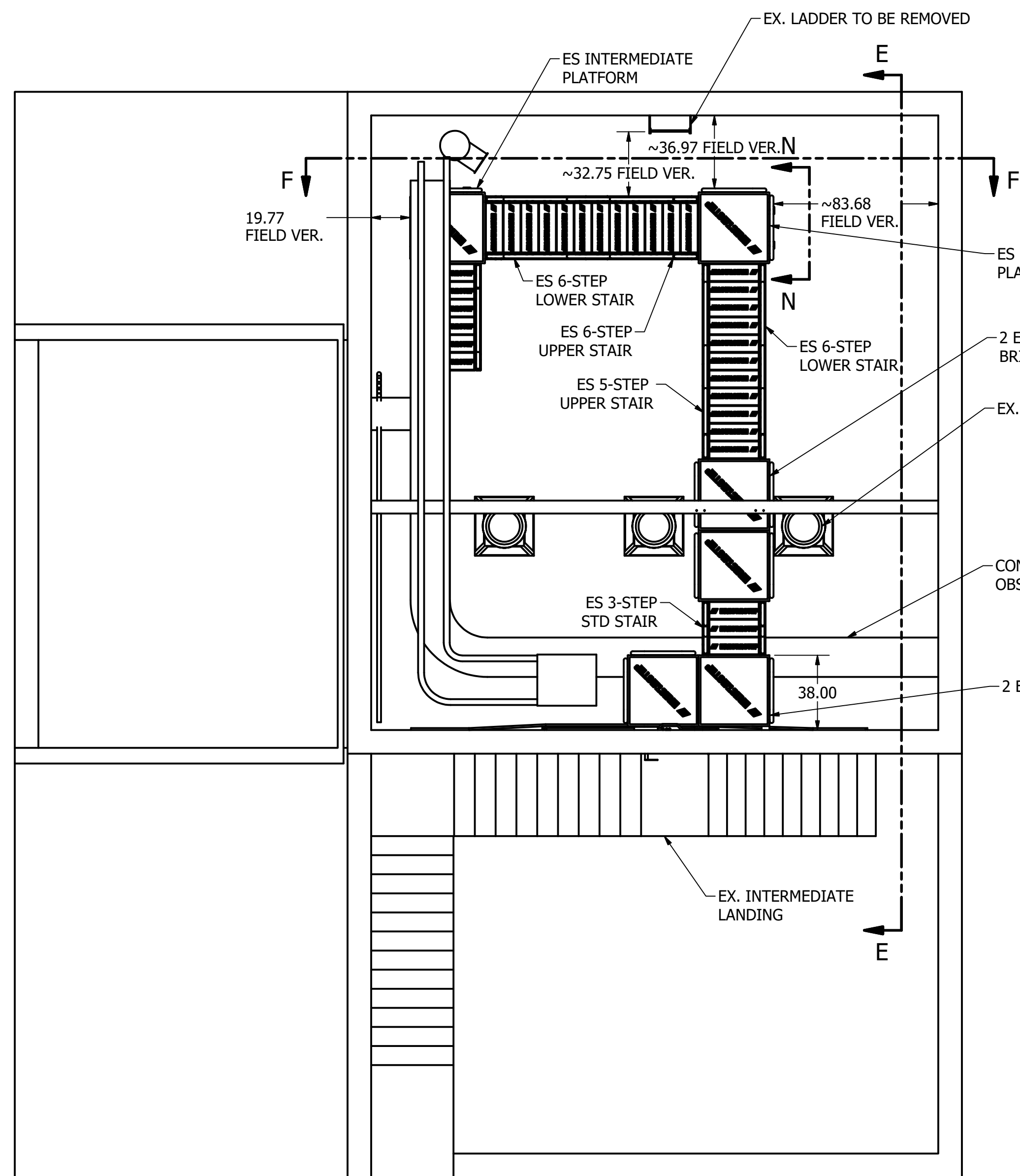
NEW STAIR PLAN
